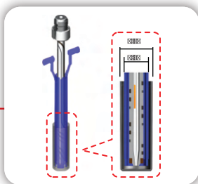
MICRO NOZZLE WITH COOLING
